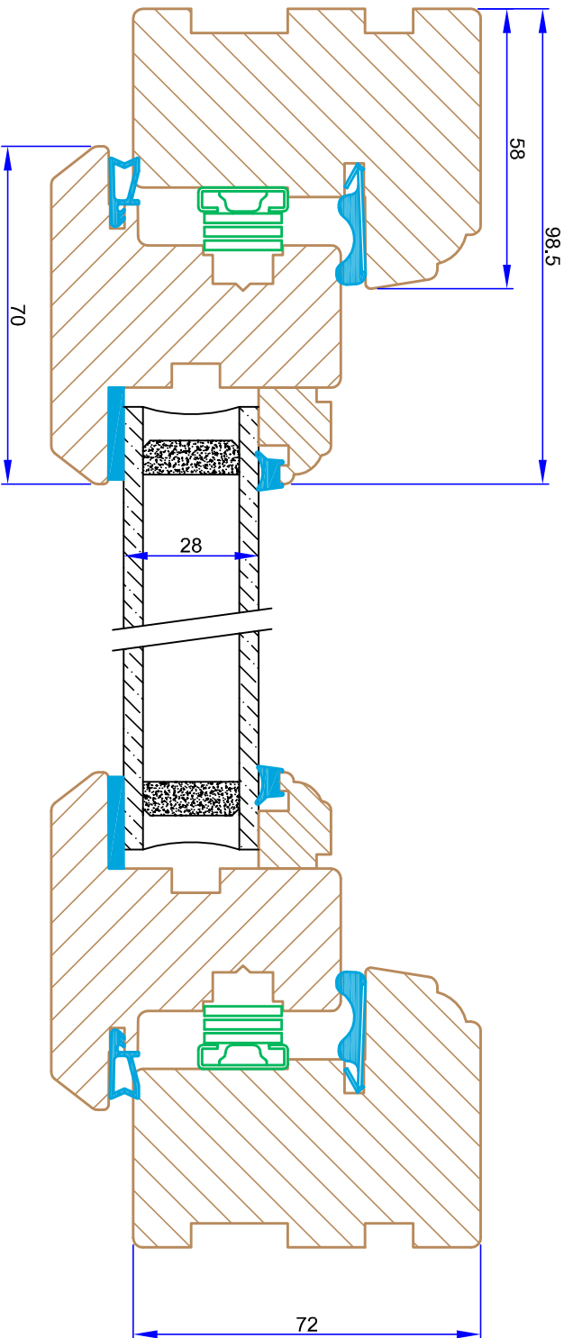
SECTION THROUGH OPENING SASH
